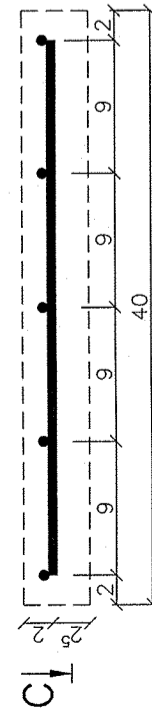
SECTION/SECTION B-B Sc.1:5
